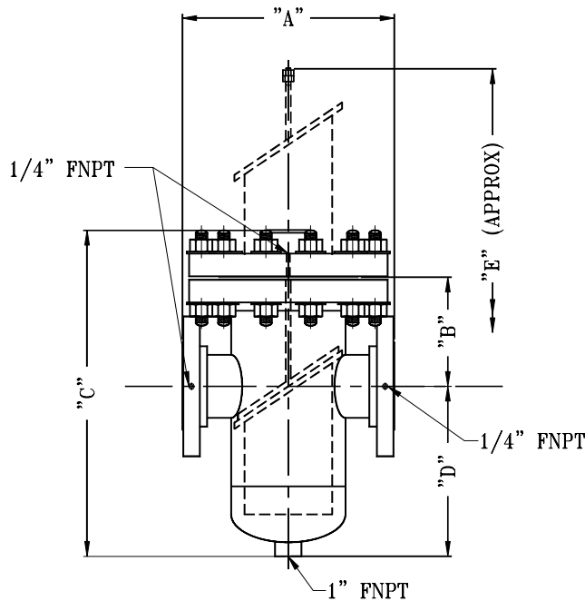
STRAINER HOUSING
